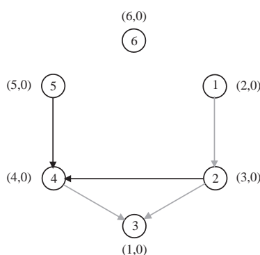
Figure 4: G^* , the result of the permutation procedure.
