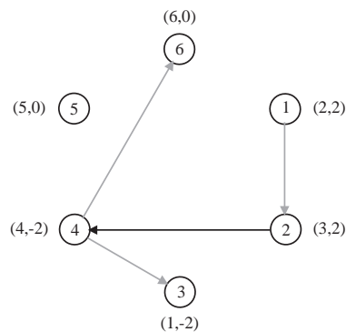
Figure 6: result of the sidepayment procedure.
