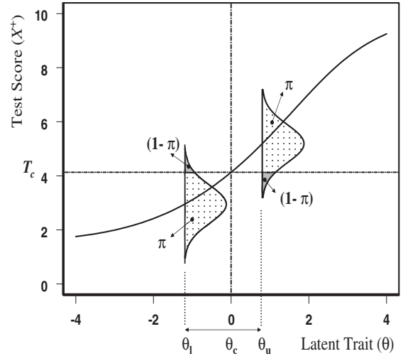
Figure 2. Distributions of test score X_+ conditional on \theta , determined such that level of classification consistency \pi identifies \theta_l (left-hand distribution) and \theta_u (right-hand distribution) given cut-score \theta_c . The S-shaped curve is the test response function.
