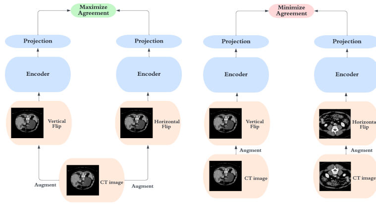
Fig. 1. Schematic overview of a contrastive learning task. Image based on [2].
