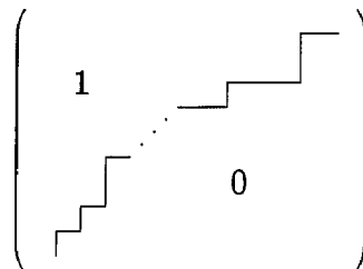
Fig. 1. A \{0,1\} matrix in echelon form.
