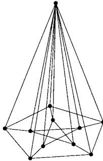
FIG. 1. The cone over the Petersen graph.
