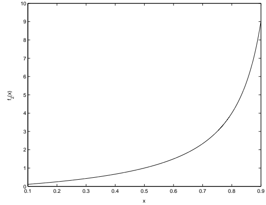
Figure 4: f_2(x) = \frac{x}{1-x} (see Kleijnen and van Beers (2004)).
